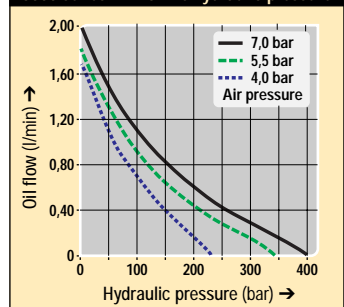
5000 series – Flow vs hydraulic pressure
