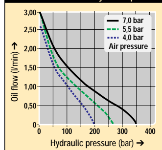
3000 series – Flow vs hydraulic pressure
